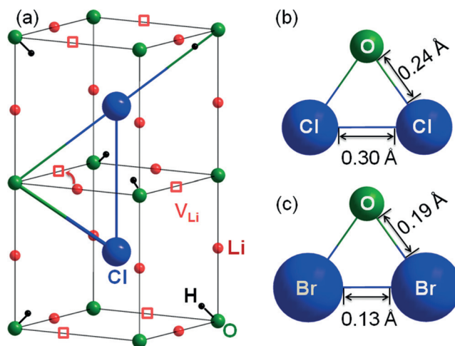
Figure 2. a) Crystal structure of cubic Li 2 OHCl; H + is on the axis of a O–Cl bond and forms an OH − bond; the triangle is the Cl–O–Cl plane in the path of Li-ion transport. Red open squares indicate Li vacancies. b), c) The size of the Cl–O–Cl triangle in cubic Li 2 OHCl and the Br–O–Br triangle in Li 2 OHBr or “Li 3 OBr”.
